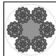
6X19 EN12385-4
