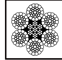
6X36 WS=6X[1+7+(7+7)+14] - IWRC COMPACTED STRAND EN12385-4 JUS C.H1.108 DIN 3064
