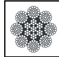
8X26 WS=8X[1+5+(5+5)+10] IWRC EN12385
