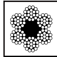
6X19 Filler=6X(1+6+6F+12) FC EN12385 JUS C.H1.086 DIN 3057
