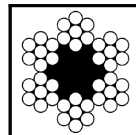
6X7=6X(1+6) FC EN12385-4 JUS C.H1.070 DIN 3055
