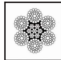
6X41 WS=6X[1+8+(8+8)+16] IWRC EN12385-4
