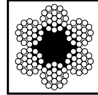
6X19 W=6X[1+6+(6+6)] FC EN12385-4 JUS C.H1.090 DIN 3059
